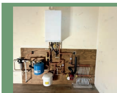
Boiler Floor Heat System
